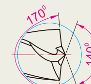
"F" Flatted Point
